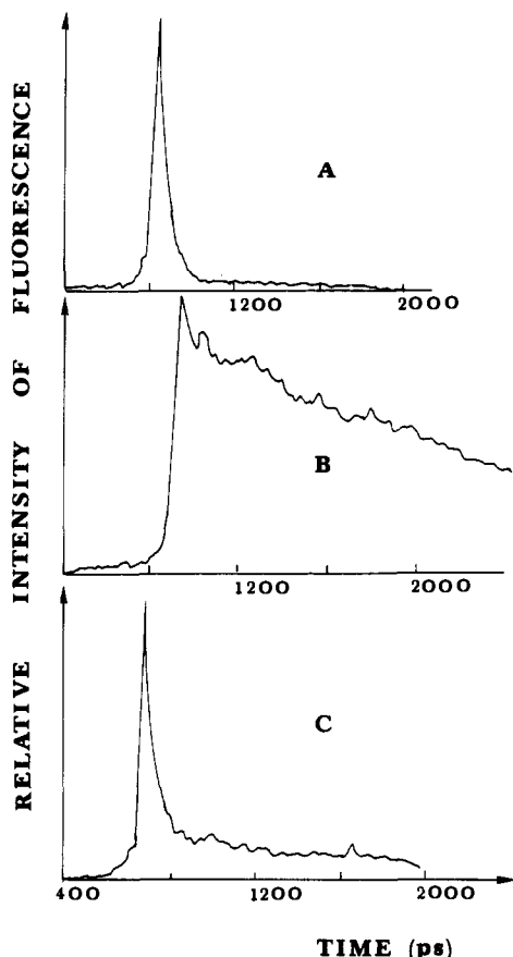
Figure 2. The fluorescence decay curves of N -methyl-2-naphthalenecarbohydroxamic acid (33) in methanol ( c \sim 10^{-6} M): (A) before irradiation; (B) after 15 min of irradiation ( \lambda_{\text{irr}} = 290 \pm 20 nm); (C) after ca. 1 h in the dark. 47
