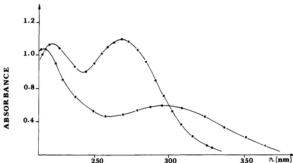
Figure 4. UV spectra of N -phenylbenzenecarbohydroxamic acid (45, 7 \times 10^{-5} M); (O) methanol; (●) methanol/NaOH aq = 1:1, pH \sim 13 . 56
