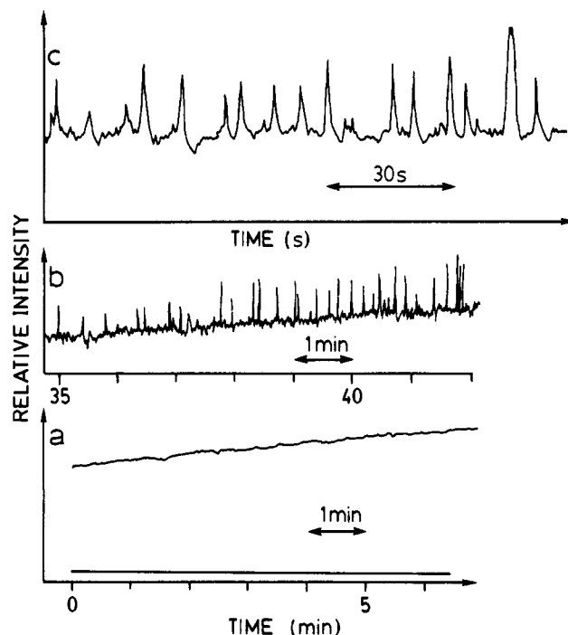
Figure 1. Plot of the fluorescence emission intensity vs time for a 6.0 \times 10^{-4}\text{ M} solution of N -methylantranilohydroxamic acid in methanol at 25\text{ }^\circ\text{C} ; \lambda_{\text{exc}} = 370 \pm 7\text{ nm} , \lambda_{\text{em}} = 425 \pm 3\text{ nm} . The base line for a and b is the bottom (solid horizontal line). The time scale of the curve c is expanded. 45
